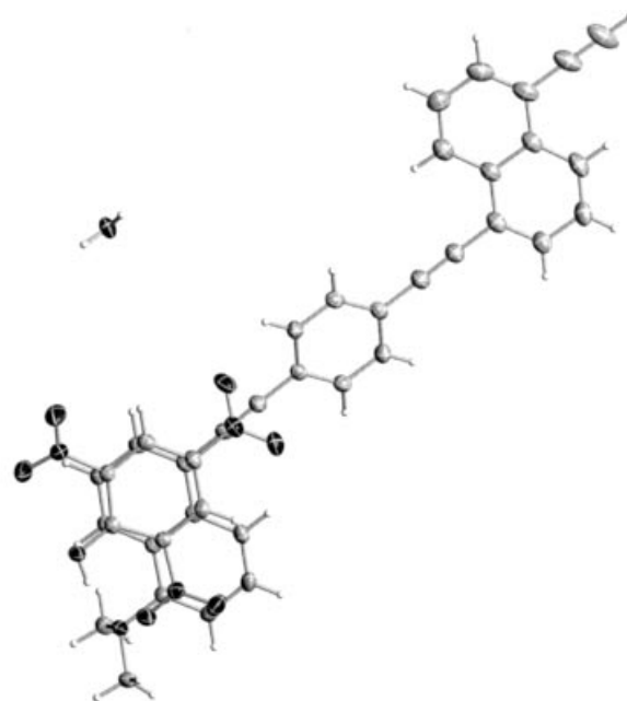
Figure 2. Molecular projection of the picrate complex of 5 along the a axis
