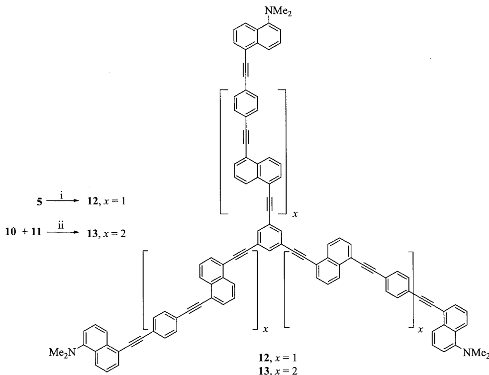
Scheme 3. (i) [\text{PdCl}_2(\text{PPh}_3)_2] , \text{Cu}_2\text{I}_2 , \text{NEt}_3 , 1,3,5-triiodobenzene; (ii) [\text{PdCl}_2(\text{PPh}_3)_2] , \text{Cu}_2\text{I}_2 , \text{NEt}_3
