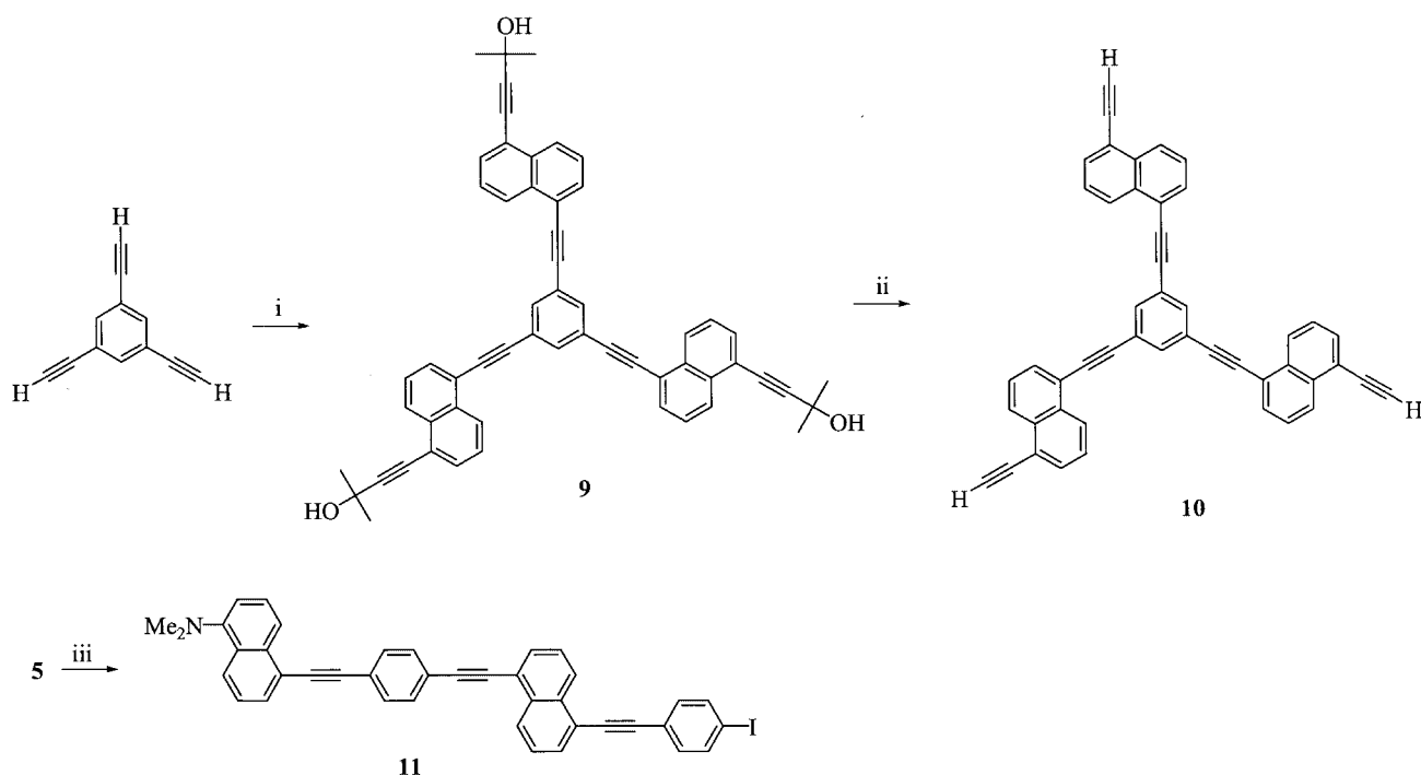
Scheme 4. (i) [\text{PdCl}_2(\text{PPh}_3)_2] , \text{Cu}_2\text{I}_2 , \text{NEt}_3 , 4-(5-iodo-1-naphthyl)-2-methyl-3-butyn-2-ol; (ii) \text{NaOH} , toluene, reflux; (iii) [\text{PdCl}_2(\text{PPh}_3)_2] , \text{Cu}_2\text{I}_2 , \text{NEt}_3 , p -diiodobenzene
