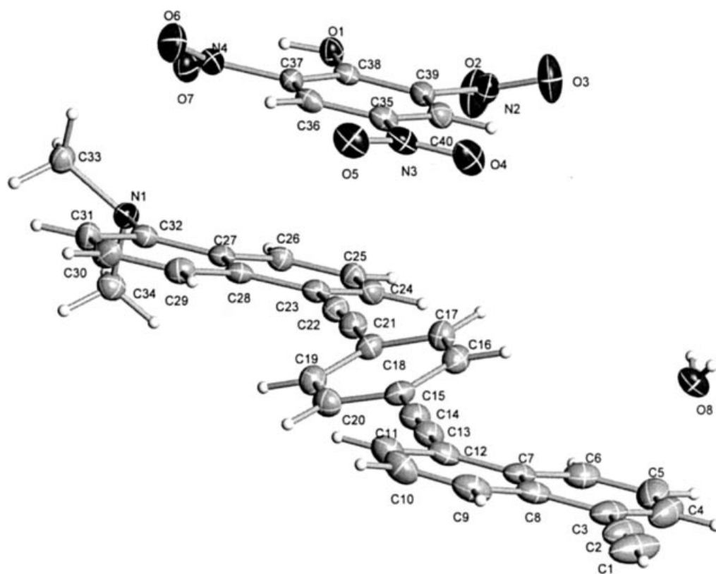
Figure 1. Molecular structure of the picrate complex of 5 (1:1 complex)
