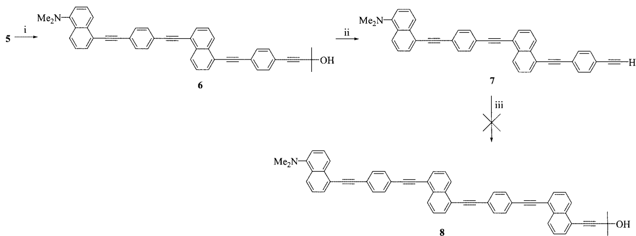
Scheme 2. (i) [\text{PdCl}_2(\text{PPh}_3)_2] , \text{Cu}_2\text{I}_2 , \text{NEt}_3 , 4-( p -iodophenyl)-2-methyl-3-butyne-2-ol; (ii) \text{NaOH} , toluene, reflux; (iii) [\text{PdCl}_2(\text{PPh}_3)_2] , \text{Cu}_2\text{I}_2 , \text{NEt}_3 , 4-(5-iodo-1-naphthyl)-2-methyl-3-butyne-2-ol
