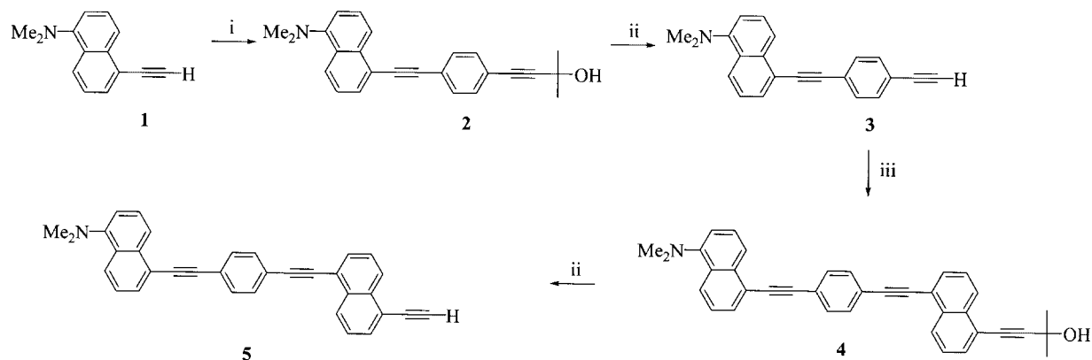
Scheme 1. (i) [\text{PdCl}_2(\text{PPh}_3)_2] , \text{Cu}_2\text{I}_2 , \text{NEt}_3 , 4-( p -iodophenyl)-2-methyl-3-butyne-2-ol, \text{CO}_2 atmosphere; (ii) \text{NaOH} , toluene, reflux; (iii) [\text{PdCl}_2(\text{PPh}_3)_2] , \text{Cu}_2\text{I}_2 , \text{NEt}_3 , 4-(5-iodo-1-naphthyl)-2-methyl-3-butyne-2-ol
